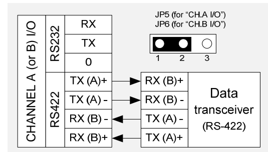
Figure 6 Data transceiver connection on RS-422 interface.
