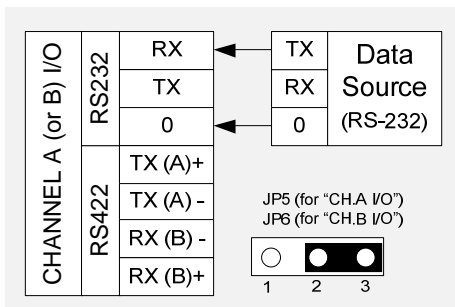
Figure 3 Data source connection on RS-232 interface.
