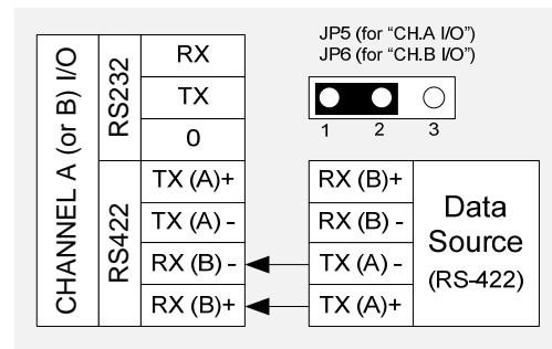
Figure 4 Data source connection on RS-422 interface.
