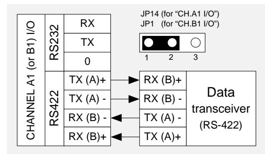
Figure 10 Data transceiver connection on RS-422 interface.
