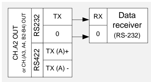
Figure 11 Data receiver connection on RS-232 interface.
