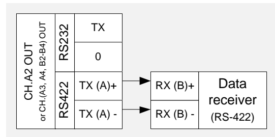
Figure 12 Data receiver connection on RS-422 interface.
