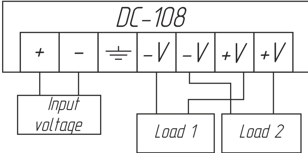
Figure 2 – The Product’s connection diagram
