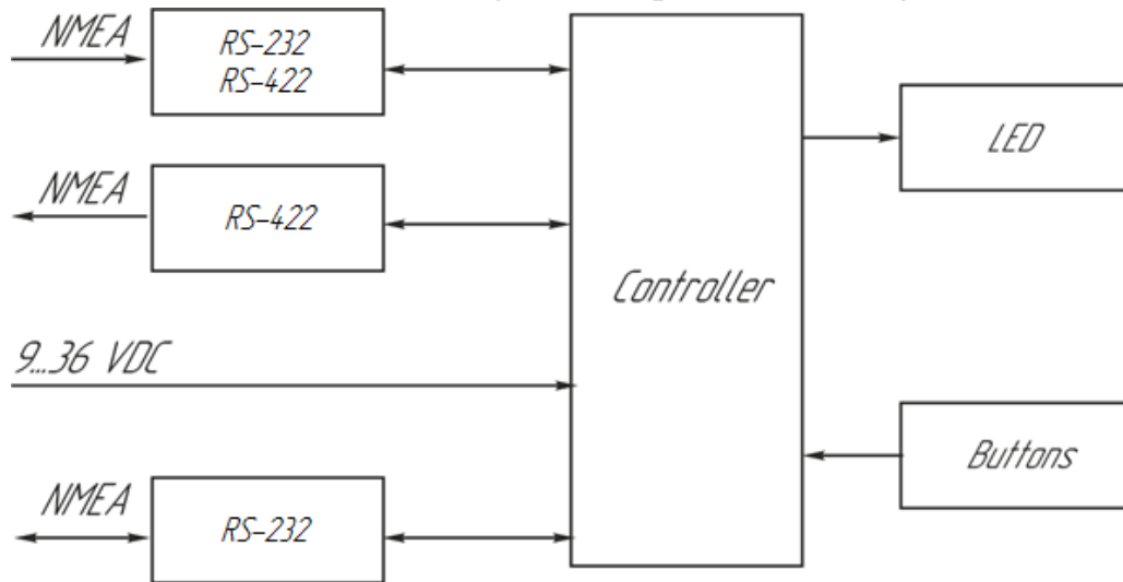
Figure 1 – Functional diagram of the Repeater
